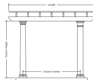
Front View Ledger runs length of pergola.
